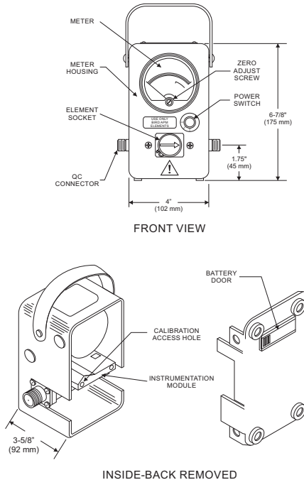
Figure 1 Outline Drawing
